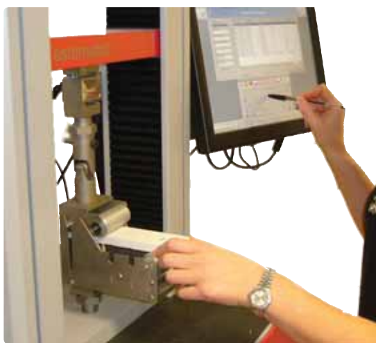
Above: Some examples of GRC flexural testing.
